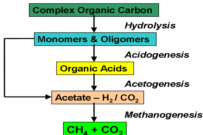
Fig 2: Reaction taking place in the anaerobic digester
